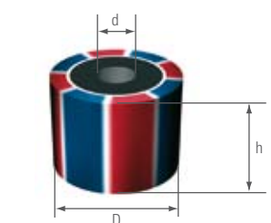
ring magnet system, magnets outside (rotor or stator for motors and radial (coaxial) couplings)
