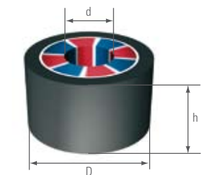
Ring magnet system, magnets inside (rotor or stator for motors and radial (coaxial) couplings)
