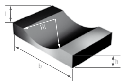
Rectangular magnet with inside radius
