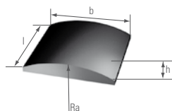
Rectangular magnet with outside radius
