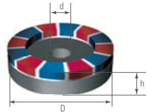
Sensor exciter ring assembly (for sensor applications such as motor commutation)
